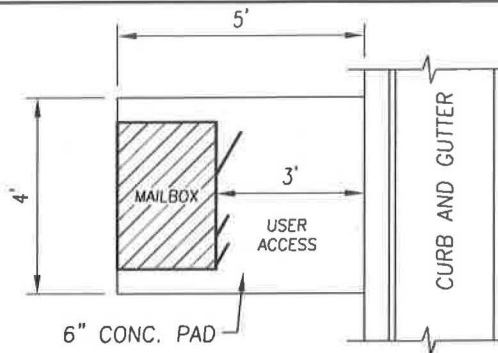
PLAN - WITHOUT SIDEWALK
