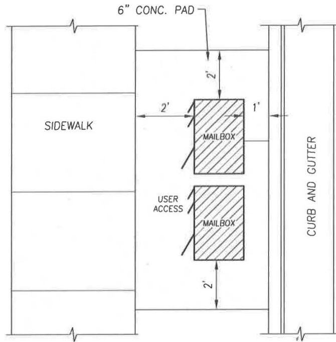
PLAN - WITH SIDEWALK
