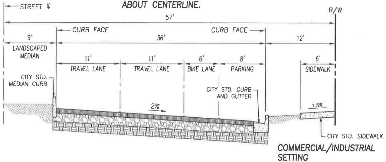
4-LANE MAJOR ARTERIAL STREET COMMERCIAL/INDUSTRIAL SETTING (114' TOTAL R/W)
