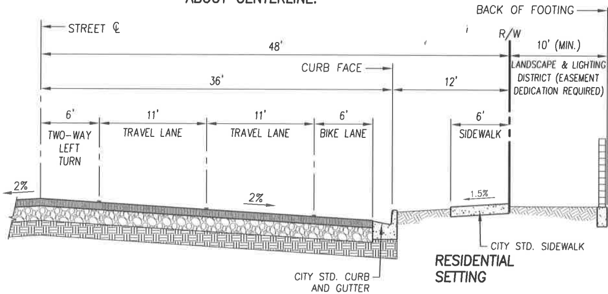
4-LANE MINOR ARTERIAL STREET RESIDENTIAL SETTING (96' TOTAL R/W)
