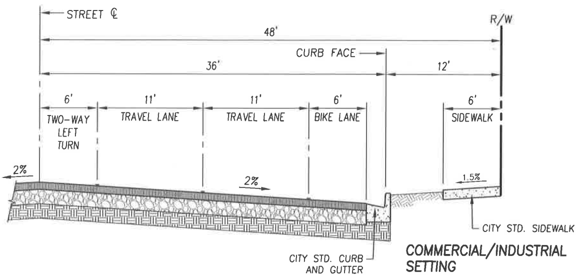
4-LANE MINOR ARTERIAL STREET COMMERCIAL/INDUSTRIAL SETTING (96' TOTAL R/W)
